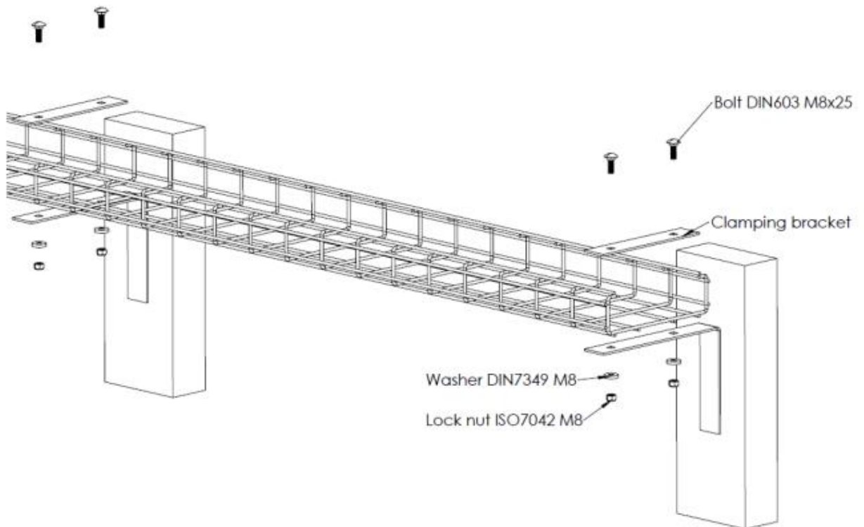
Figure 2 - Clamping to wall brackets
